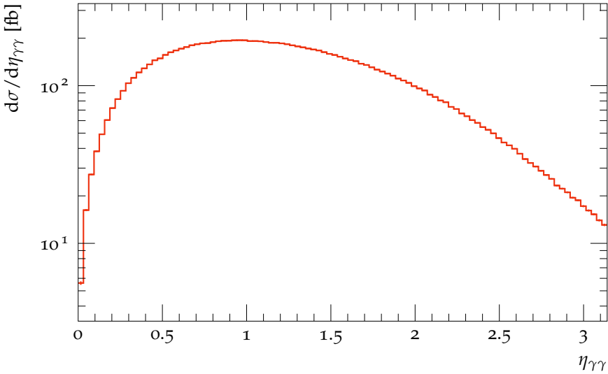
Rapidity of diphoton system
