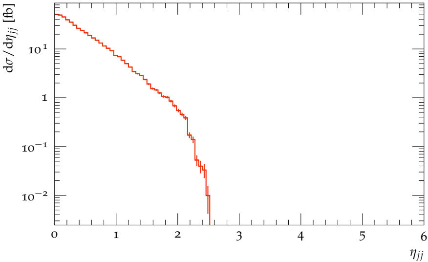
Rapidity of system of two hardest jets
