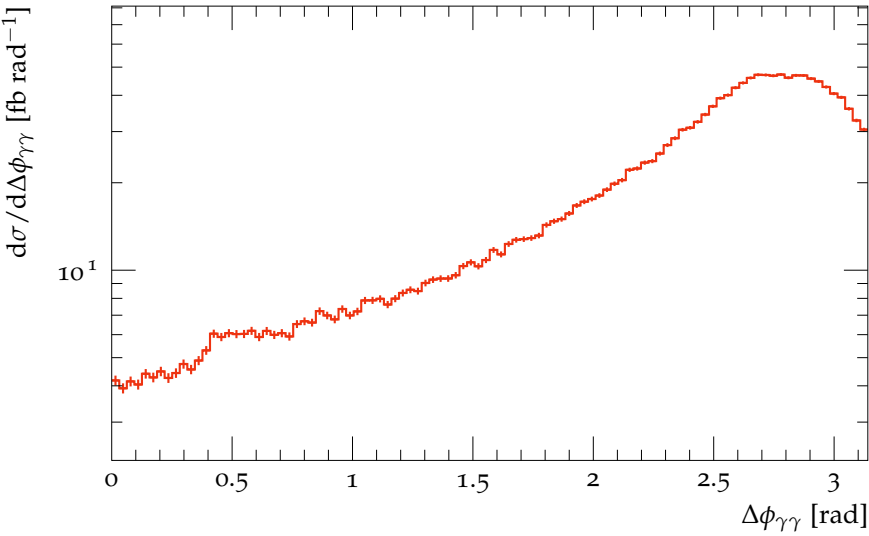
Azimuthal angle between the photons
