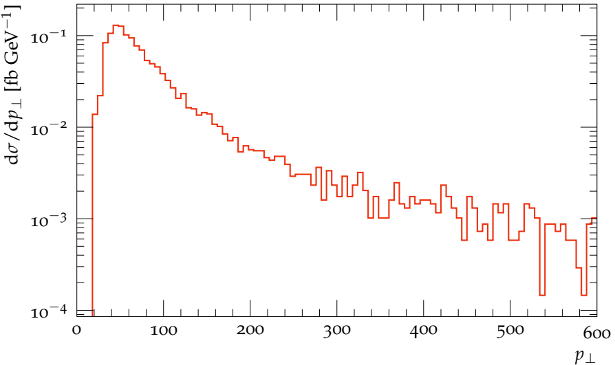
Transverse momentum of second hardest jet
