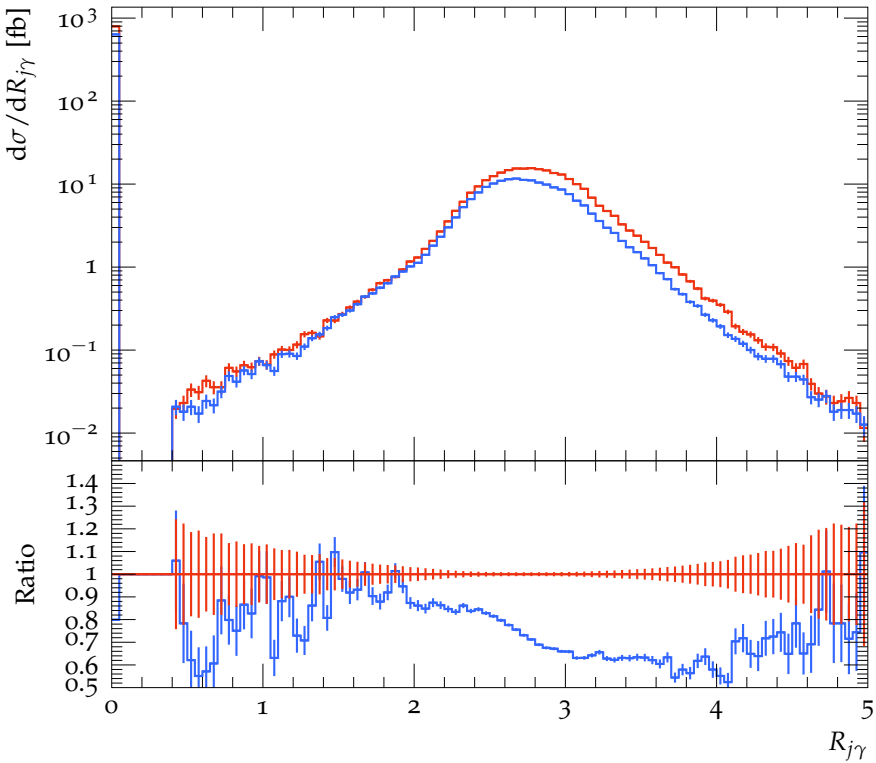
R-separation between hardest jet and hardest photon
