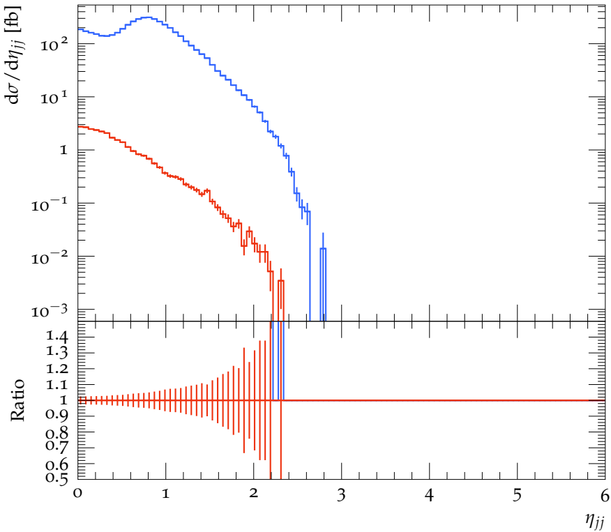
Rapidity of system of two hardest jets
