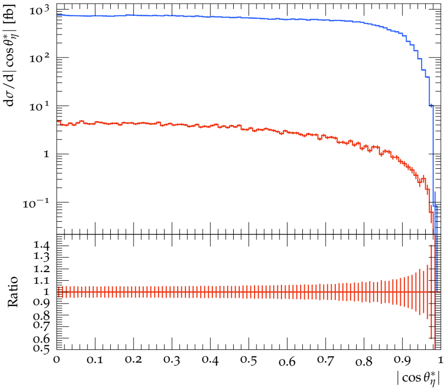
Polar scattering angle of the photons
