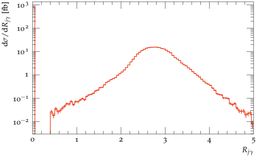
R-separation between hardest jet and hardest photon
