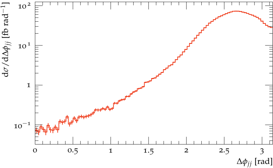
Azimuthal angle between the two hardest jets
