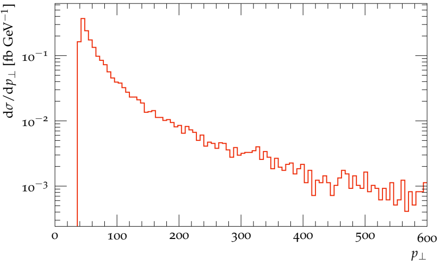
Transverse momentum of hardest jet
