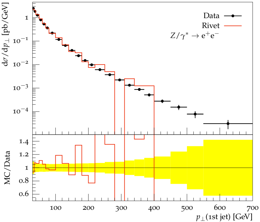
Transverse momentum of 1st jet
