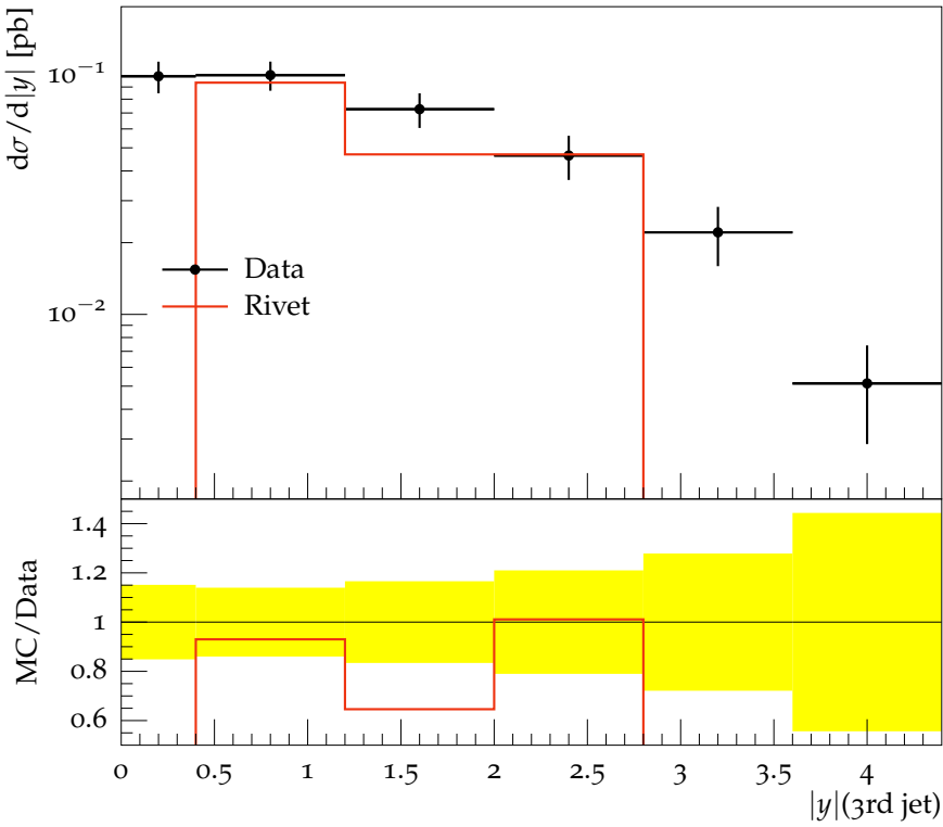
Rapidity of 3rd jet (VBF selection)
