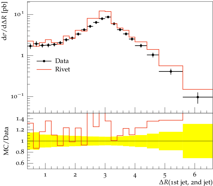
\Delta R distance of leading jets
