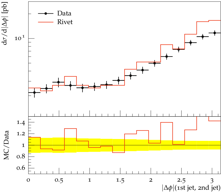
Azimuthal distance of leading jets
