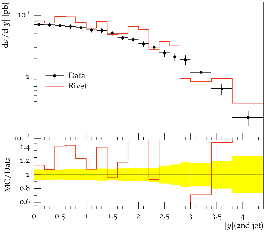
Rapidity of 2nd jet
