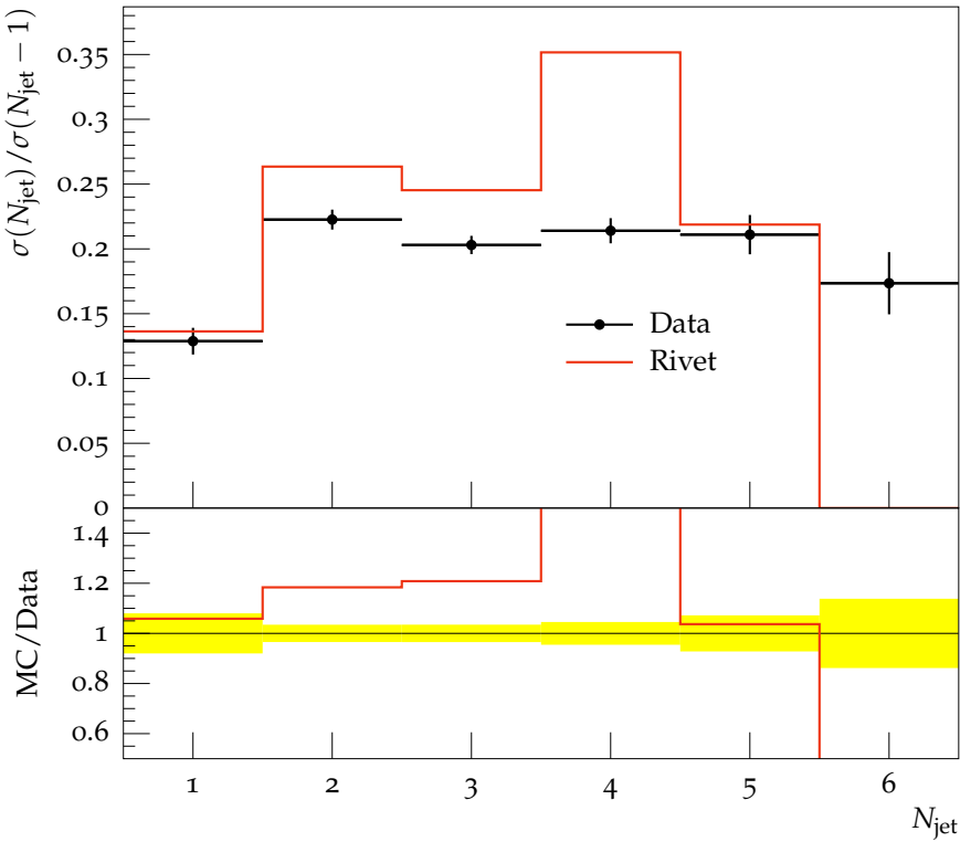
Exclusive jet multiplicity ratio
