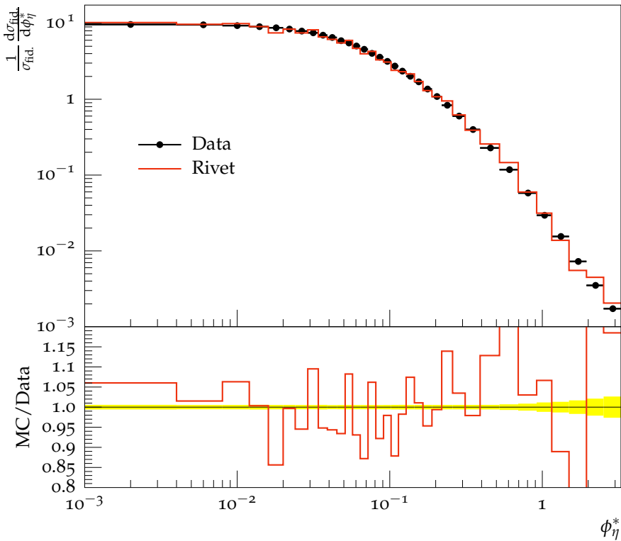
\phi_\eta^* spectrum, Z \rightarrow ee (dressed)
