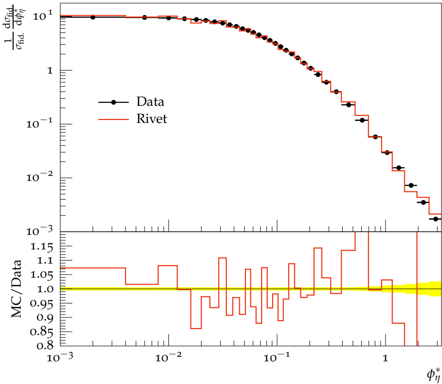
\phi_\eta^* spectrum, Z \rightarrow ee (bare)
