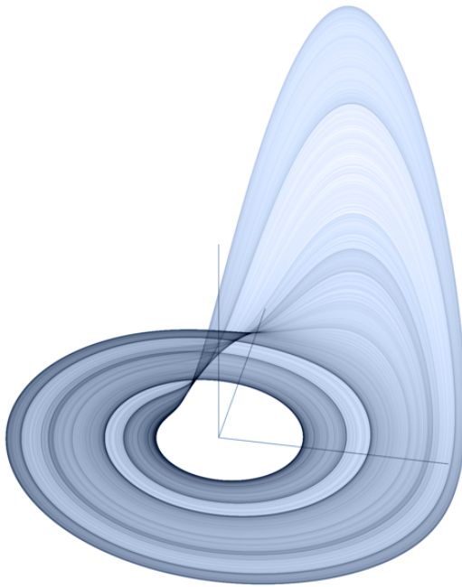
Figure 7.1: The Roessler attractor
