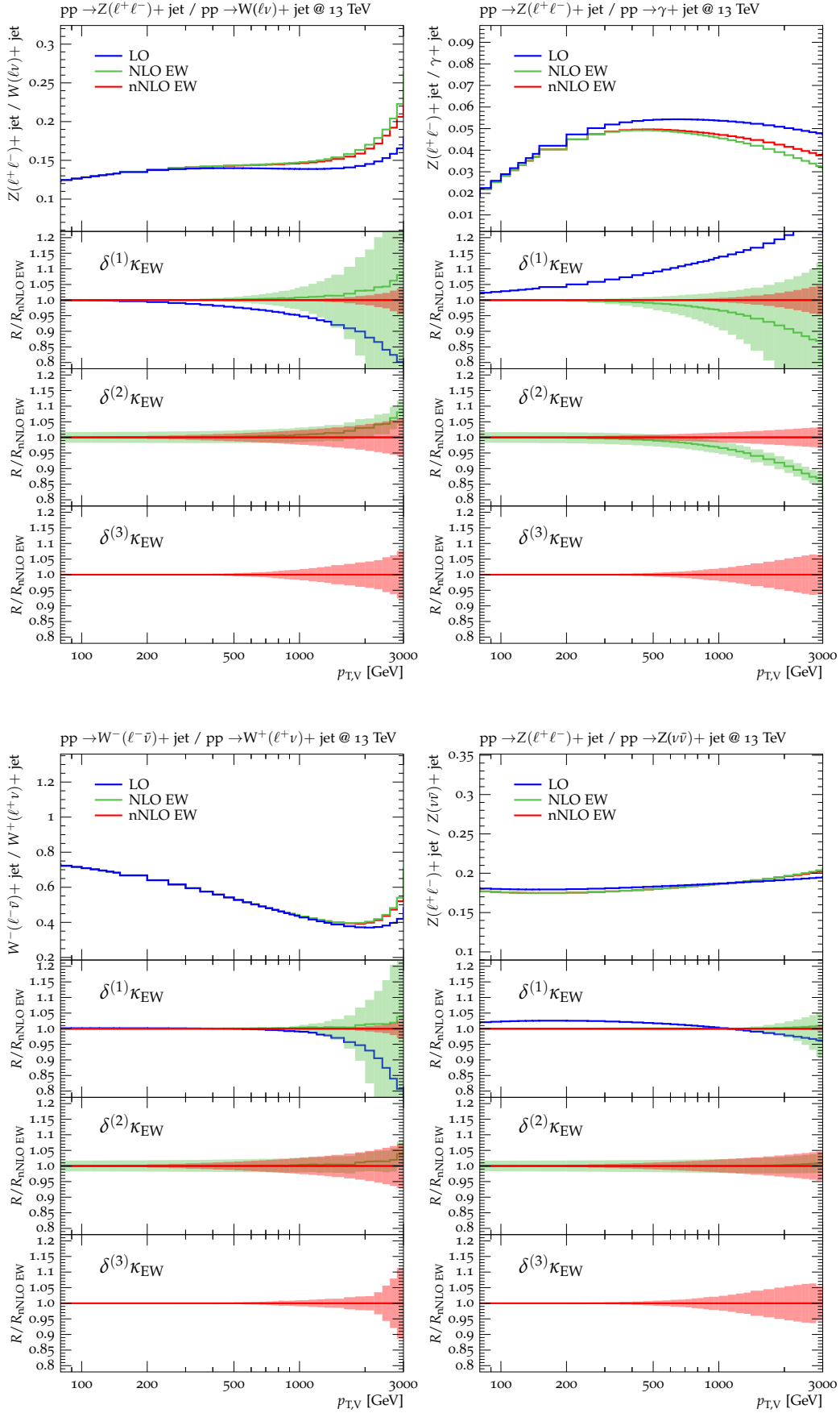
Fig. 21: Ratios of p_T -distributions for various pp \rightarrow V + \text{jet} processes at LO, NLO EW and nNLO EW. The related EW uncertainties, \delta^{(i)}\kappa_{EW}^{(V)} , are defined in Eqs. (52), (53) and (56) at nNLO and in Eq. (57) at NLO. The uncertainty \delta^{(1)}\kappa_{EW}^{(V)} is correlated amongst processes, while \delta^{(2)}\kappa_{EW}^{(V)} and \delta^{(3)}\kappa_{EW}^{(V)} are uncorrelated.
