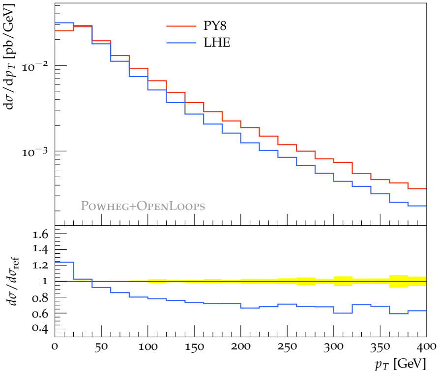
p_T of the t\bar{t}b\bar{b} system (ttbb cuts)
