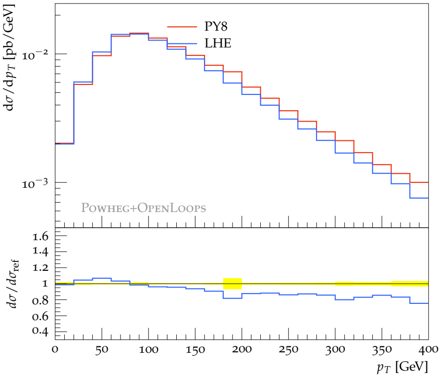
p_T of the t\bar{t} system (ttbb cuts)
