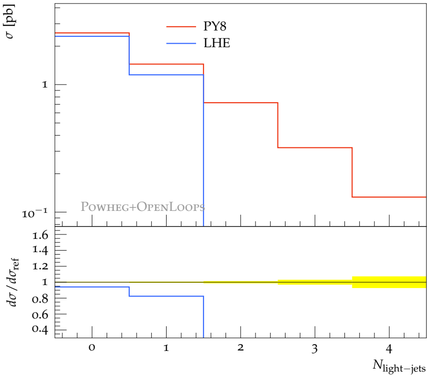
Inclusive light-jet multiplicity distribution (ttbb cuts)
