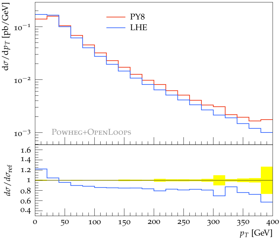
p_T of the t\bar{t}b system (ttb cuts)
