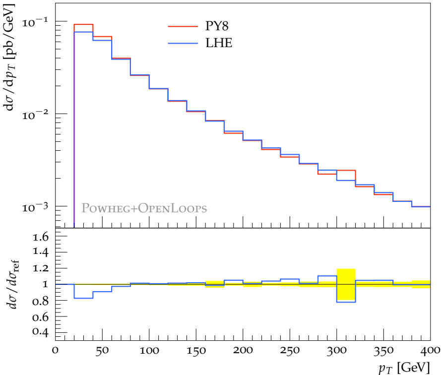
p_T of 1 st light-jet (ttb cuts)
