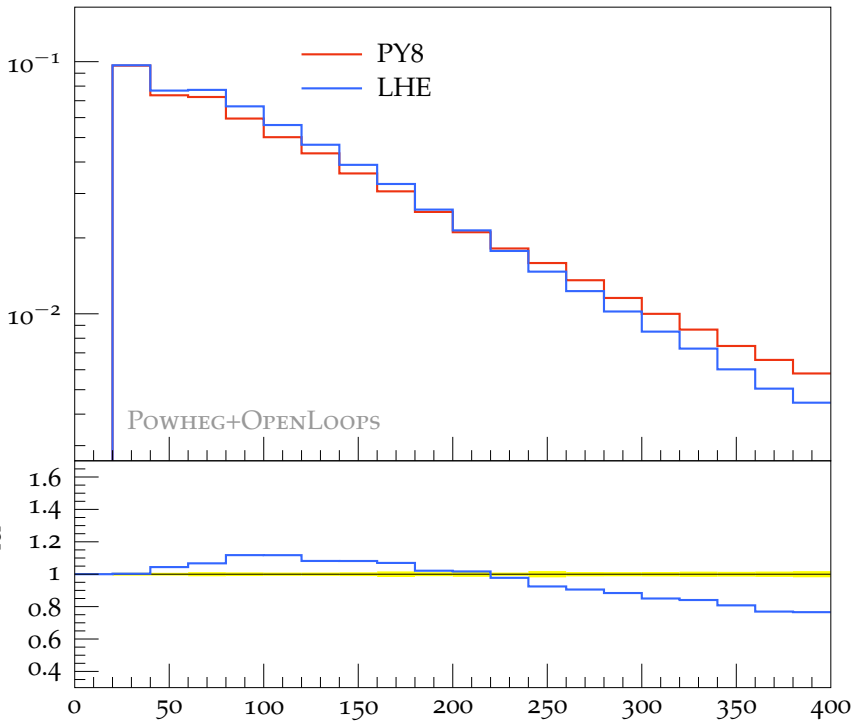
Sum of p_T of all reconstructed jets (ttb cuts)
