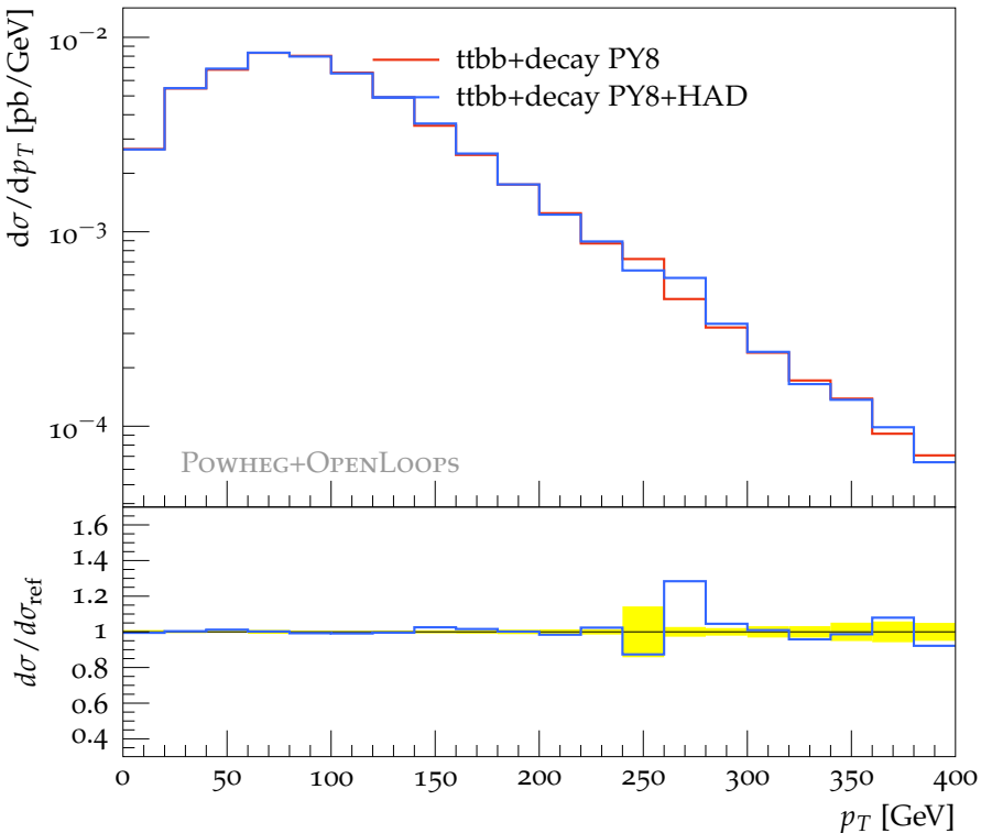
p_T of 2 nd and 3 rd b-jet pair (WW 3 b cuts)
