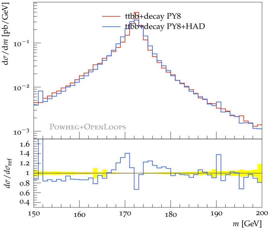
Mass of best b -jet- W (anti)top candidates (WW 4 b cuts)
