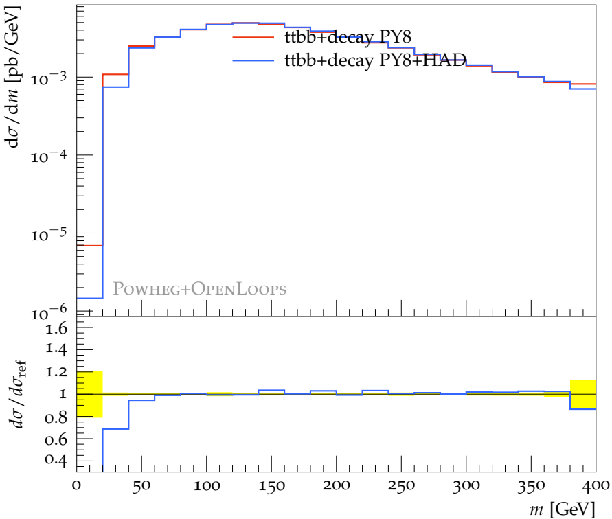
Invariant mass of the 1 st and 3 rd b-jets (WW 4 b cuts)
