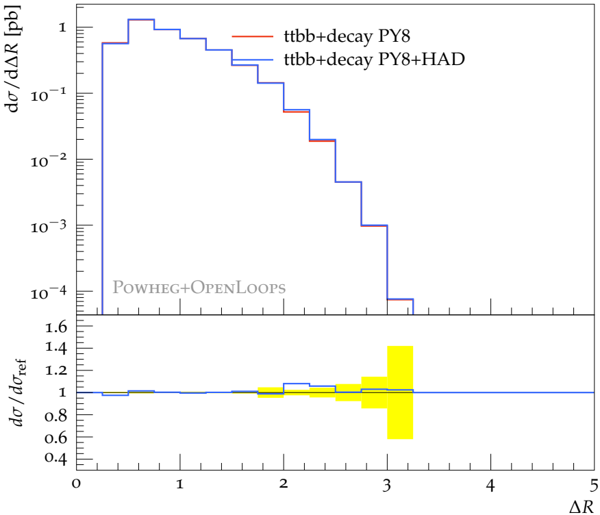
min \Delta R of the four hardest b-jets (WW 4 b cuts)
