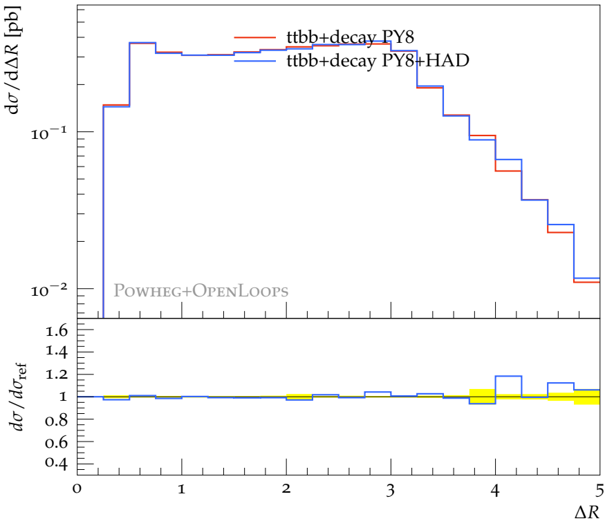
\Delta R of 3 rd and 4 th b-jets (WW4b cuts)
