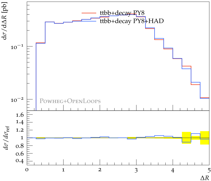
\Delta R of 2 nd and 4 th b-jets (WW 4 b cuts)
