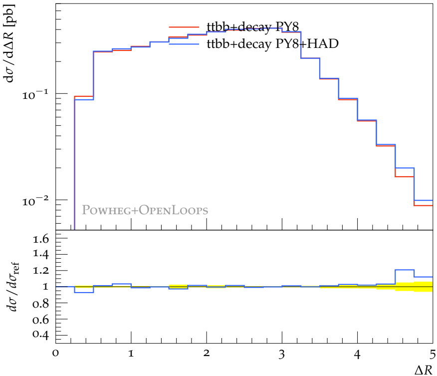
\Delta R of 2 nd and 3 rd b-jets (WW 4b cuts)
