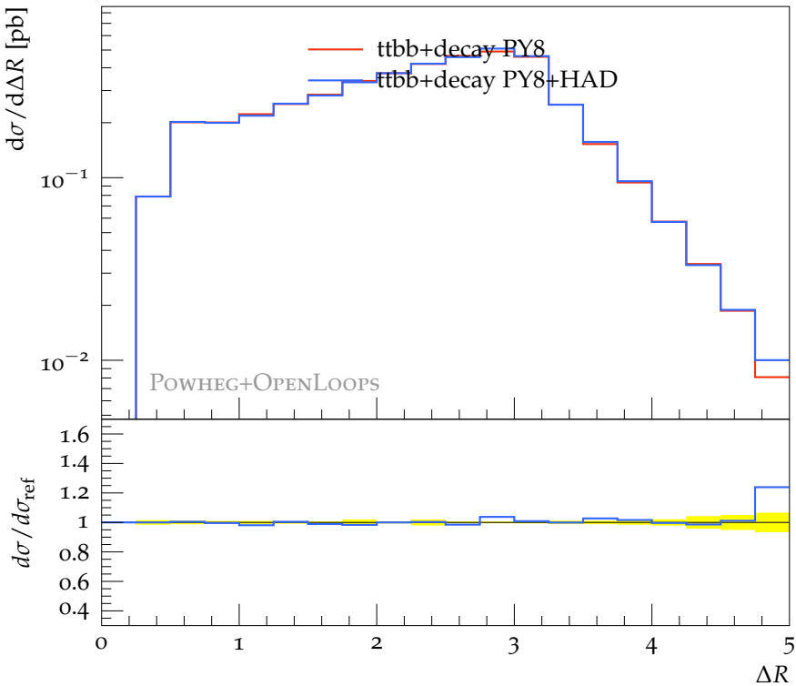
\Delta R of 1 st and 3 rd b-jets (WW4b cuts)
