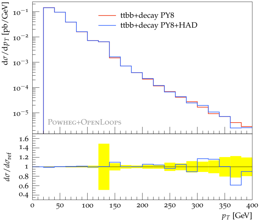
p_T of 3 rd b-jet (WW3b cuts)
