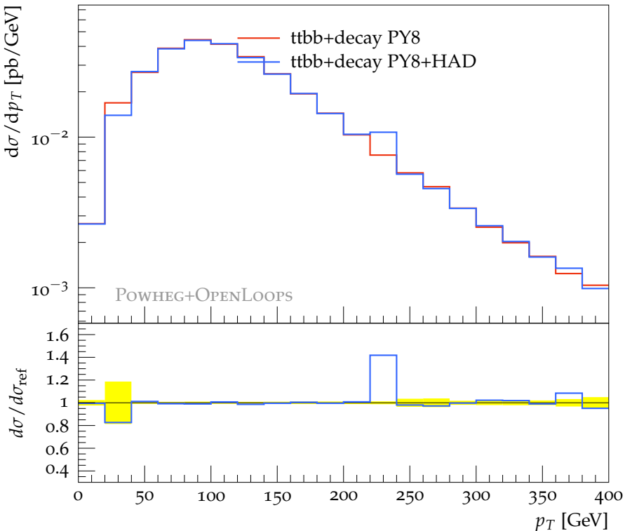
p_T of 1 st and 3 rd b-jet pair (WW 3 b cuts)
