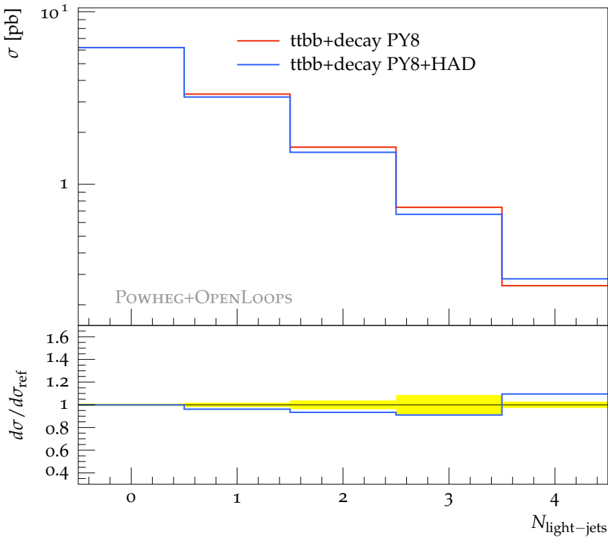
Inclusive light-jet multiplicity distribution (WW 3b cuts)
