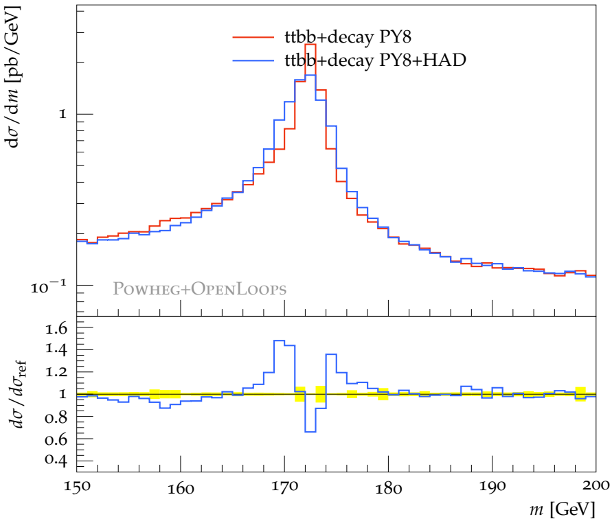
Mass of all b -jet- W pairs (WW3b cuts)
