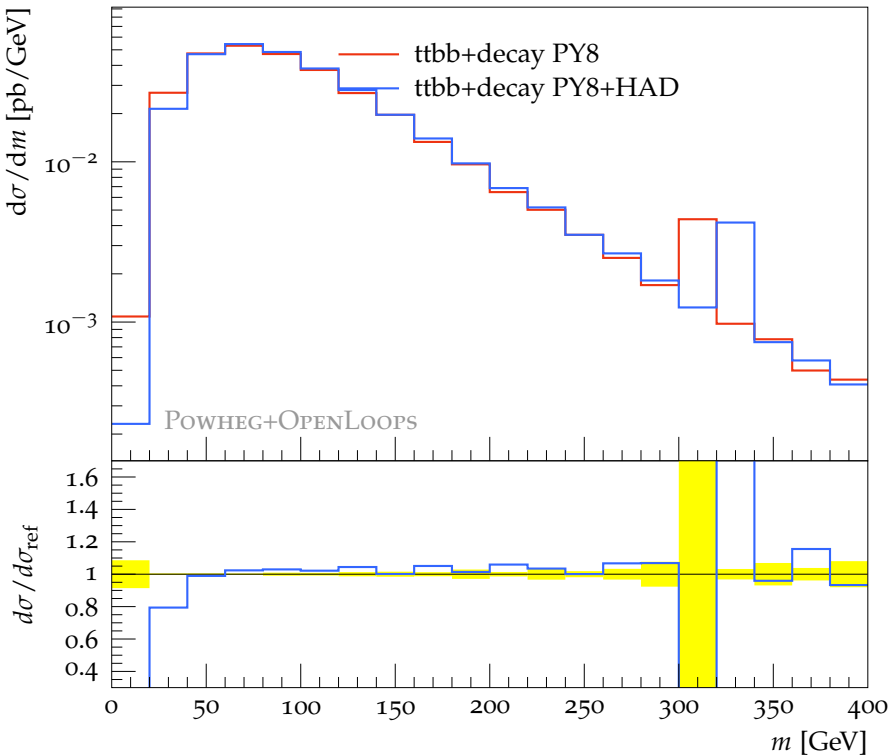
Min inv. mass of all systems of the four hardest b-jets (WW3b cuts)
