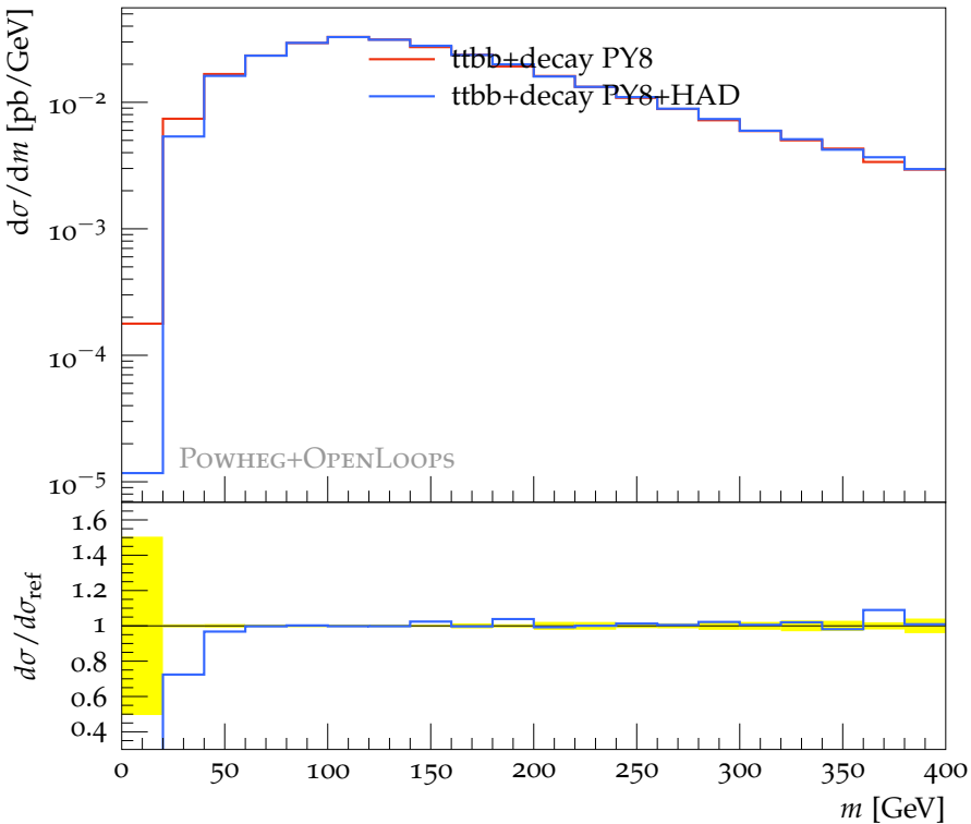
Invariant mass of the 1 st and 3 rd b-jets (WW 3 b cuts)
