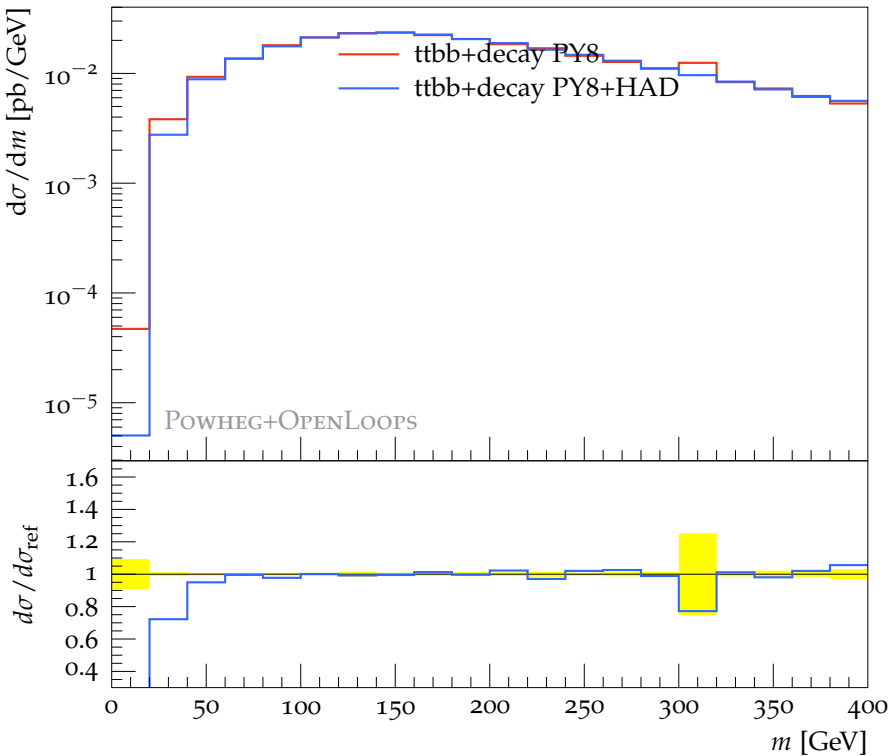
Invariant mass of the 1 st and 2 nd b-jets system (WW 3 b cuts)
