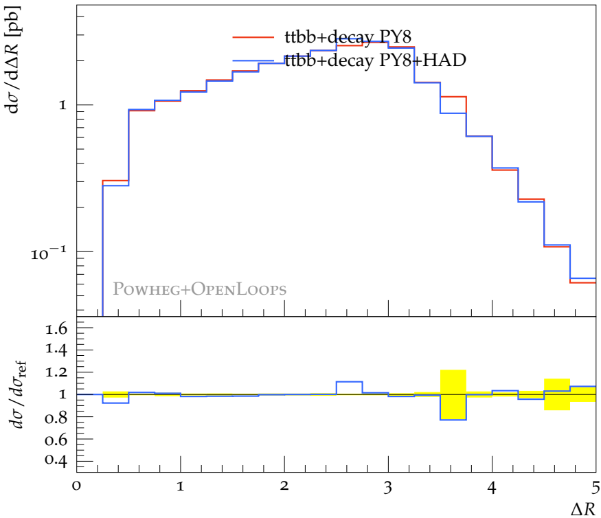
\Delta R of 1 st and 3 rd b-jets (WW 3b cuts)
