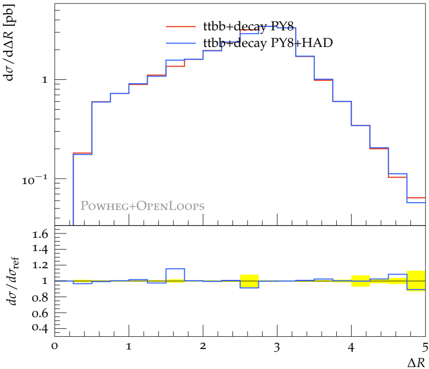
\Delta R of 1 st and 2 nd b-jets (WW 3b cuts)
