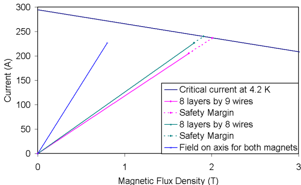
FIG. 8: (Color) Undulator conductor load lines.
