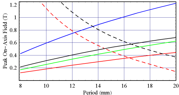
FIG. 3: (Color) Peak on-axis magnetic flux density for APPLE-II (solid, red), APPLE-III (green), multi-mode (solid, black) and PM ring undulator (blue) models in circular polarizing mode and the required period/field to produce 10 MeV photons with 150 GeV electron beam (dashed, red) and 20 MeV photons with a 250 GeV beam (dashed, black) at the first harmonic.
