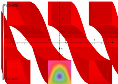
FIG. 7: (Color) Field in conductor windings, (highest field pink).
