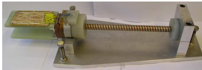
FIG. 10: (Color) Photo. of the completed SC undulator before field measurement, with twenty 14 mm periods.
