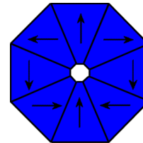
FIG. 2: (Color) Schematic showing the magnetization vectors of a dipole ring comprising of 8 magnet blocks.
