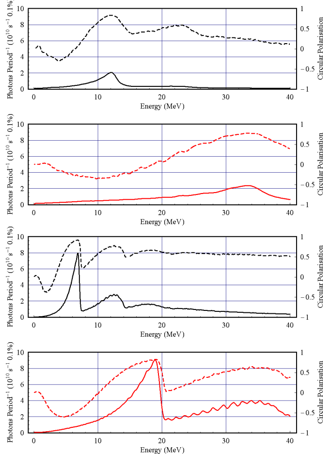
FIG. 13: (Color) Photon spectrum per period (solid) and circular polarization rate (dashed) from PM ring undulator (top) and SC undulator (bottom) for 150 GeV (black) and 250 GeV (red) Energy electrons. Calculated using the measured magnetic flux density data.
