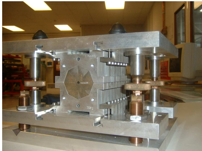
FIG. 6: (Color) Photo. of completed PM ring undulator assembly, with ten 14 mm periods.
