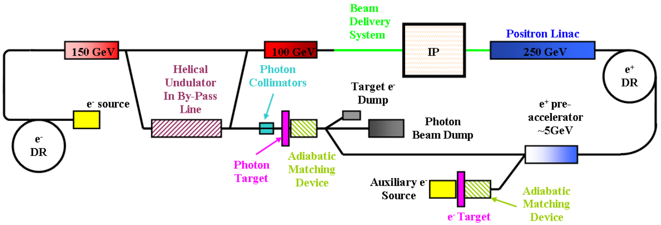
FIG. 1: (Color) ILC schematic layout with main positron source components.
