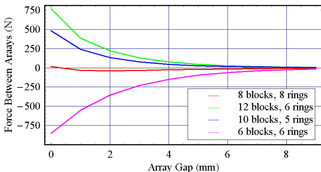
FIG. 4: (Color) Magnetic forces for 10 periods of different PM ring undulator configurations.
