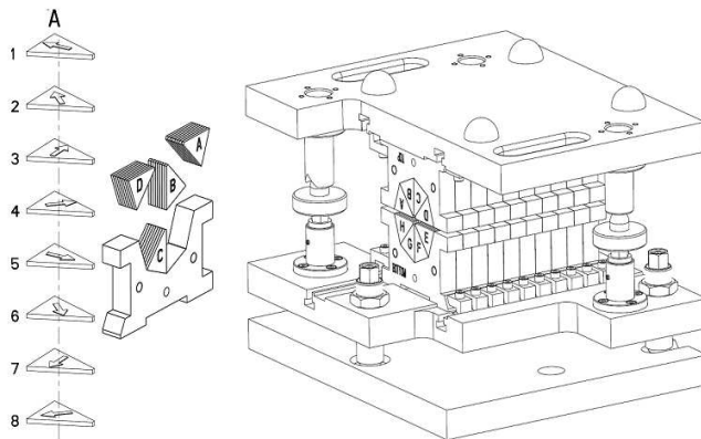
FIG. 5: Assembly drawing of PM ring undulator.
