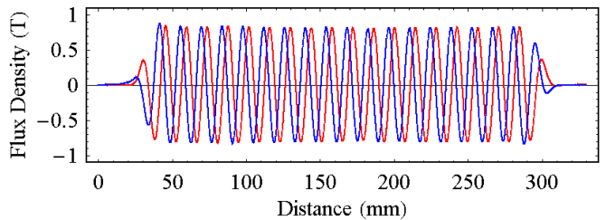
FIG. 12: (Color) Measured on-axis magnetic flux density in both transverse directions for the SC undulator.
