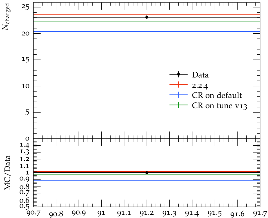
Charged particle multiplicity, b events
