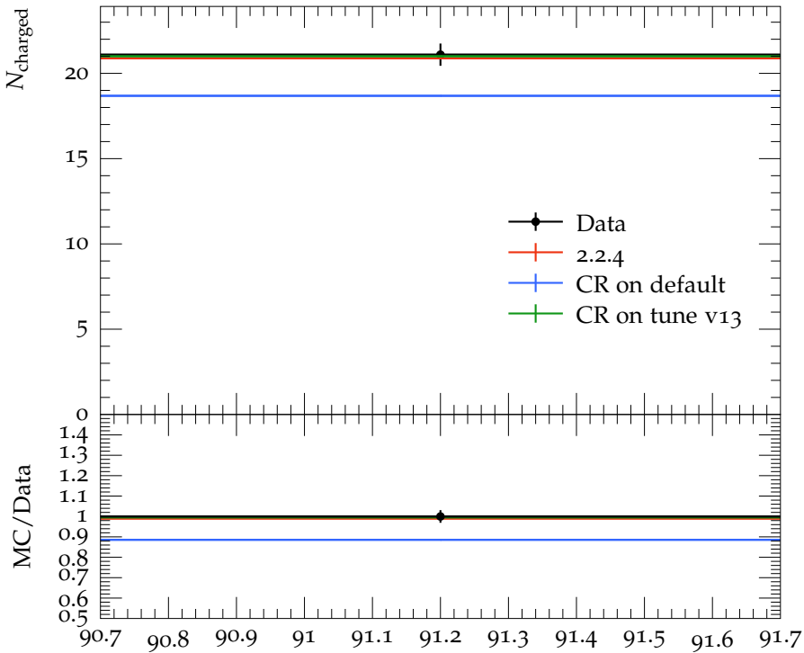
Charged particle multiplicity, c events
