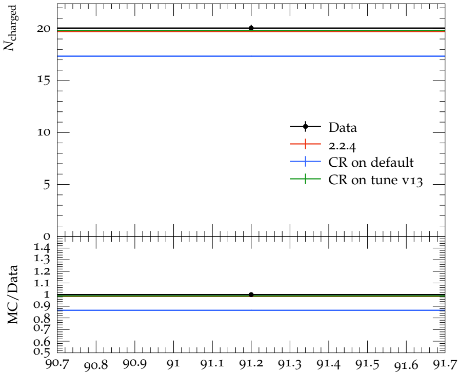
Charged particle multiplicity, ( uds ) events
