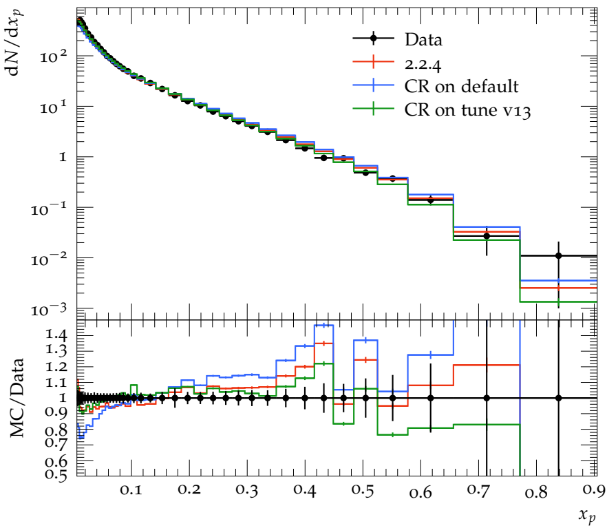
Charged particle scaled Momentum, c events
