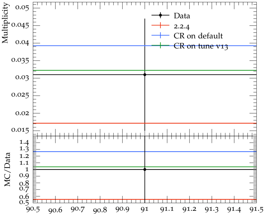
Mean \Lambda_b^0 multiplicity
