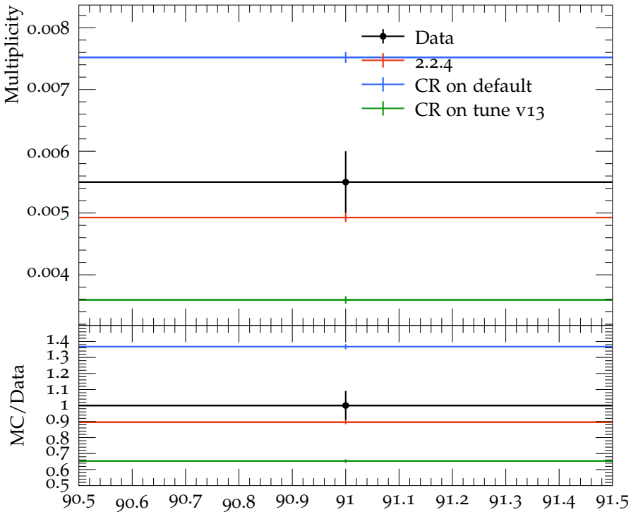
Mean \Xi^0(1530) multiplicity
